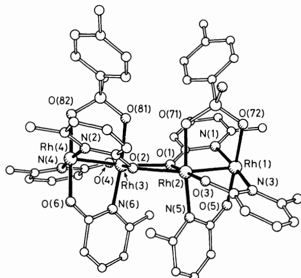
Figure 1. Molecular structure of (4). Crystals are monoclinic, a = 9.014(2) , b = 23.488(4) , c = 27.336(9) Å, \beta = 99.08(2)^\circ , U = 5715.1 Å 3 , Z = 4 , D_c = 1.716 g cm -3 , space group P2_1/c ; crystal size ca. 0.25 \times 0.03 \times 0.03 mm. Intensities were measured to 2\theta_{\text{max}} = 42^\circ with Mo- K_\alpha radiation ( \lambda = 0.71069 Å) on a Stoe-Siemens AED diffractometer. For 3709 unique reflections with F > 3\sigma(F) , anisotropically refined atoms, and isotropic H atoms in calculated positions, R = 0.096 . Selected bond lengths (Å): Rh(1)–Rh(2) 2.377(3), Rh(3)–Rh(4) 2.376(3), Rh(2)–O(1) 2.05(1), Rh(3)–O(2) 2.02(1), Rh(2)–O(3) 2.02(1), Rh(3)–O(4) 2.02(1), Rh(1)–O(5) 1.99(1), Rh(4)–O(6) 1.99(1), Rh(3)–O(1) 2.24(1), Rh(2)–O(2) 2.30(2), Rh(1)–N(1) 2.05(1), Rh(4)–N(2) 2.05(1), Rh(1)–N(3) 2.04(1), Rh(4)–N(4) 2.04(1), Rh(2)–N(5) 2.03(1), Rh(3)–N(6) 2.05(1), Rh(2)–O(71) 2.11(1), Rh(1)–O(72) 2.11(1), Rh(3)–O(81) 2.12(1), Rh(4)–O(82) 2.06(1).
